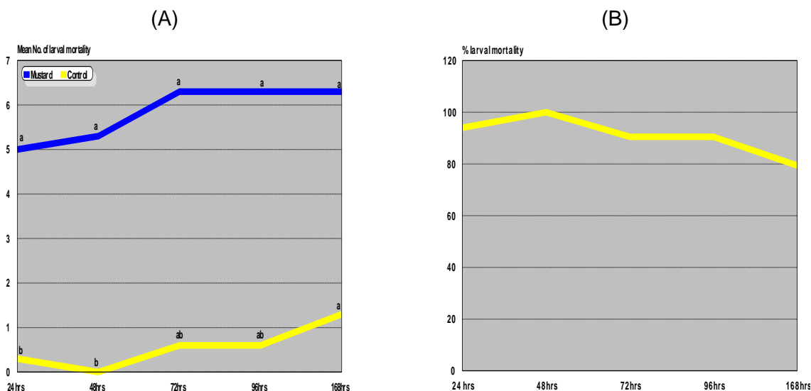
Figure (3): Effect of soil amended with mustard on the mean number (A) and percentage of larval mortality (B) of M. javanica under laboratory conditions.
